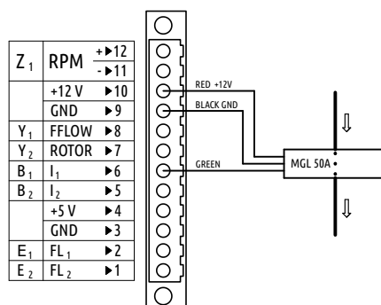
Figure 30: MGL 50A Close Loop sensor connection schematics.
