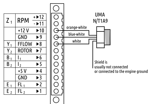
Figure 38: Connection of UMA T1A9 or N1A9 sensor to Y channel. Any Y channel can be used.
