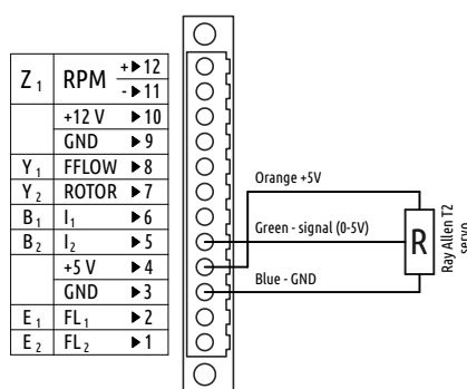
Figure 36: Direct connection to Ray Allen T2 servo.
