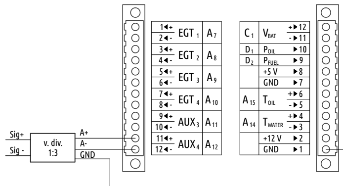
Figure 29: Voltage adapter 1:3 is connected to the A channel.
