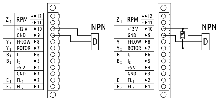
Figure 14: Left: a typical example of NPN digital sensor connection. Right: In some cases an external pullup resistor is needed.
