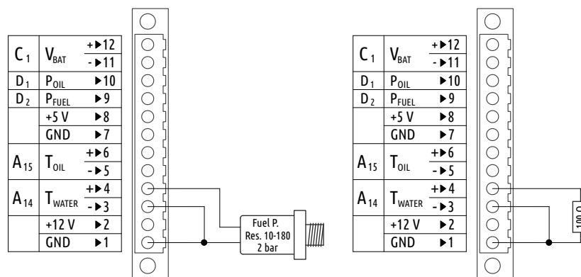
Figure 47: Example: VDO 2 bar sensor was replaced by a fixed 100 Ohm resistor.
