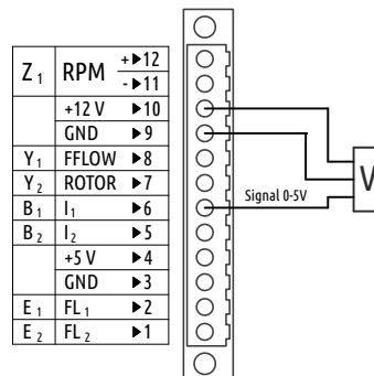
Figure 10: An example of active sensor with voltage output.
