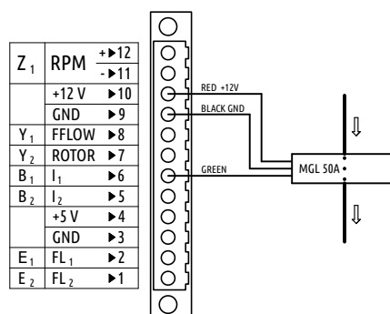
Figure 33: MGL 50A Close Loop sensor connection schematics.
