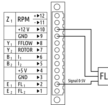
Figure 35: An example of capacitive fuel level probe connected to the +12 V power source. Some probes require 5 V, be careful.
