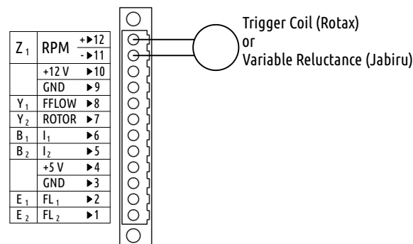
Figure 37: Connection of trigger coil sensor or variable reluctance sensor to Z channel.
