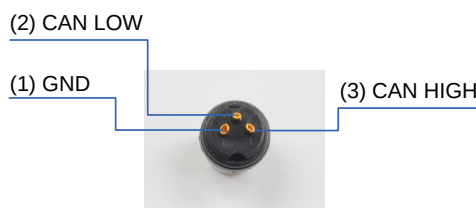
Figure 44: Photo of connector back side. Note the three small numbers, which define the pin positions. GND is usually not connected.
