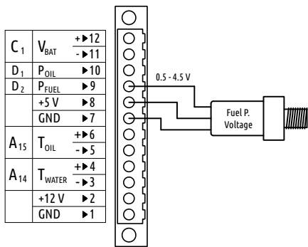
Figure 25: Fuel pressure sensor with variable voltage (0.5 – 4.5 V) output. Sensor is powered with 5V.
