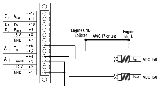
Figure 19: Typical oil and coolant (water) sensor connection. One wire principle is used for the oil sensor and two wire principle for the coolant sensor.
