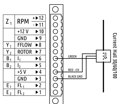
Figure 31: Current Hall 30/60/100 sensor connection schematics.
