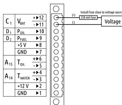
Figure 27: System voltage measurements. A 250 mA (or less) fuse is required close to the system bus source.
