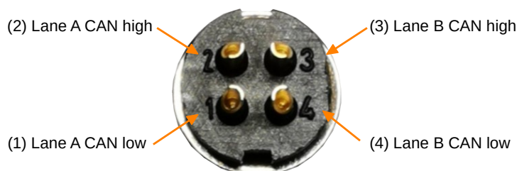
Figure 45: Cable plug back side. Note the four small numbers, which define the pin positions inside the plug. This is Binder part number 99 0979 100 04.
