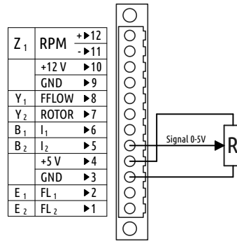
Figure 13: An example of potentiometer, connected as variable voltage divider.
