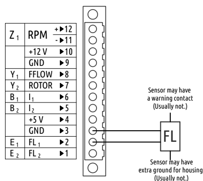
Figure 34: An example of resistive fuel sensor. Usually it has only two connections. But it can have more. Please refer to the sensor manual for more details.
