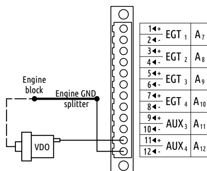
Figure 23: VDO oil pressure sensor with one wire principle. The second wire is hidden and connects via engine block.
