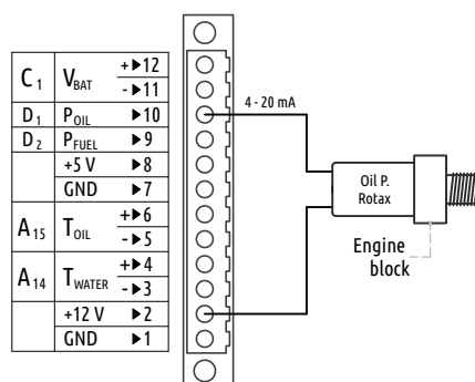
Figure 21: Typical oil pressure sensor connection for Rotax engine. Active, current variable sensor is used.
