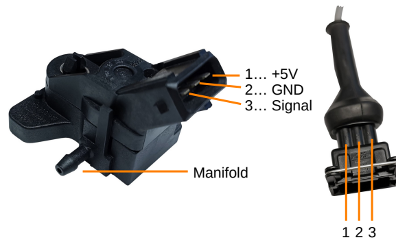
Figure 40: External manifold pressure sensor, Bosch 0 261 230 037.
