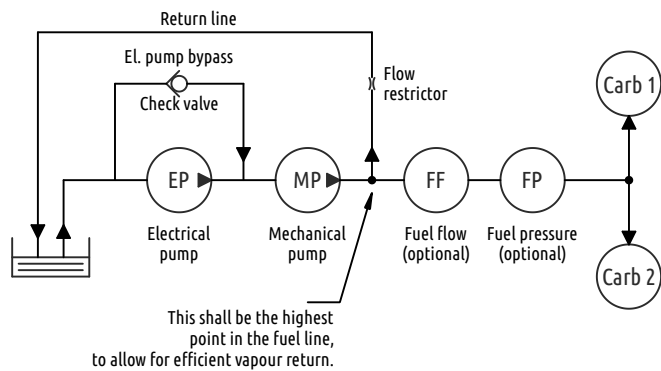
Figure 24: Recommended positions for fuel pressure and fuel flow sensors on Rotax 912 engines with two carburetors.
