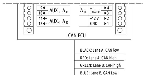
Figure 46: Color codes of the 4-pin connector. Two lanes can be connected, each has two wires. Some engines connect only one lane. WMFly Engine - CCM module, for example.
