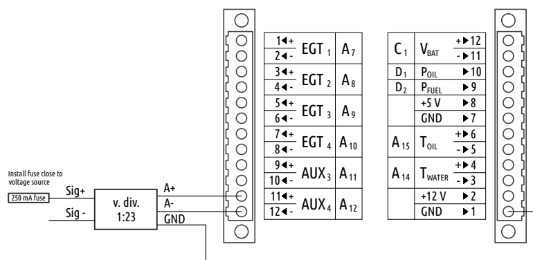
Figure 28: Voltage adapter is connected to the A channel.
