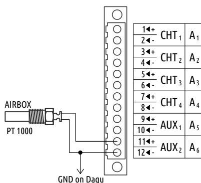
Figure 20: Typical connection of Airbox sensor with PT1000 sensing element.
