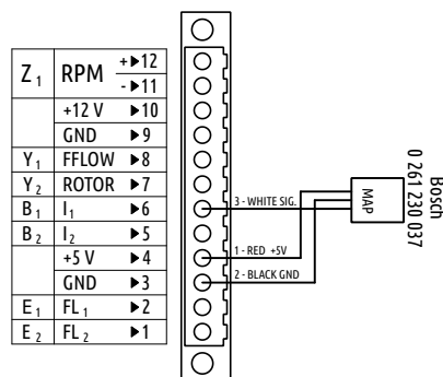
Figure 41: External MAP sensor from Bosch, connection schematics.
