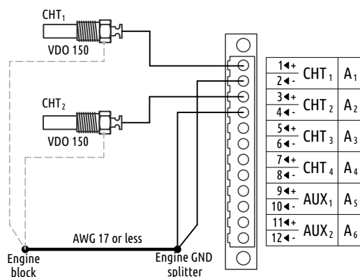
Figure 18: Typical connection of CHT sensors on Rotax 912 engines.
