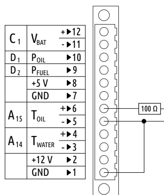
Figure 49: Example: VDO oil temperature sensor was replaced by a known test resistor. A 100 \Omega resistor is shown, but any other test resistor from Table 40 can be also used.
