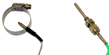
Figure 16: Hose clamp type EGT probe (left), bayonet type EGT probe (right).
