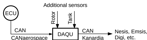
Figure 42: Illustration of the connection principle. Almost all information comes from the ECU. Rotor RPM and fuel tanks and other additional sensors can be still connected directly to Daqu.
