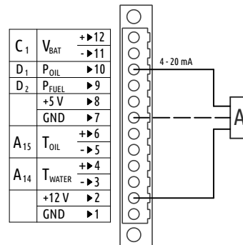
Figure 11: An example of active sensor with current output. Symbol A stands for Ampere which is synonym for electrical current. For some sensors, connection with GND is not required.
