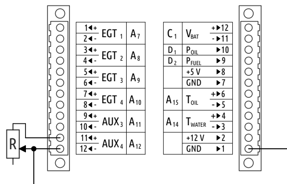
Figure 12: An example of potentiometer, connected as variable resistor.
