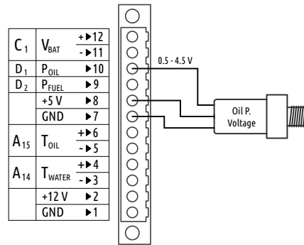
Figure 22: Oil pressure sensor with variable voltage (0.5 – 4.5 V) output. Sensor is powered with 5V.
