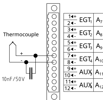
Figure 9: Thermocouples filter capacitor wiring.
