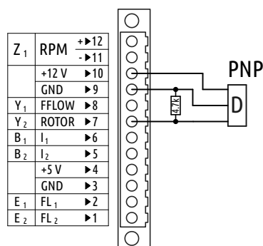
Figure 15: An example of PNP digital sensor connection. Use/experiment with 1.0–4.7 kOhm resistor.
