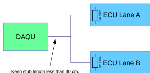
Figure 43: CAN bus connectivity.
