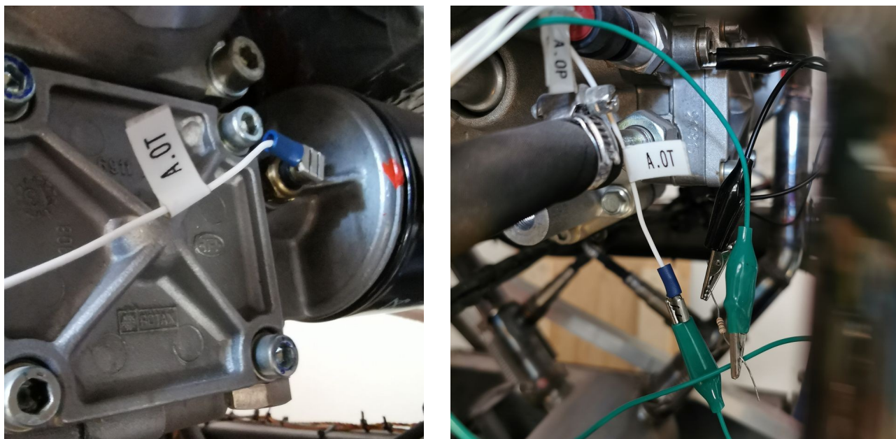
Figure 48: Test setup. Left: Location of the oil temperature sensor and its lead to Daqu (labeled as A.OT). Right: Oil temperature lead was detached and connected with green cable to one side of the test resistor. The other side of the resistor connects to an appropriate engine point (black cable).
