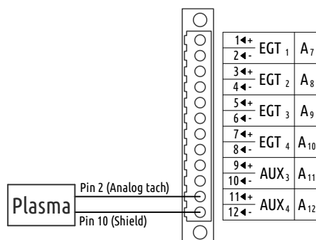
Figure 39: Connection of Plasma RPM analogue voltage output signal to A channel.
