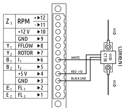
Figure 32: CT-30 sensor connection schematics.
