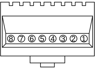
Front view RJ45 connector
