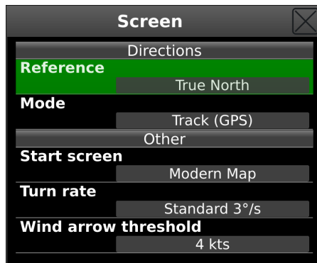
Figure 30: Parameters related to the Aetos screens.
