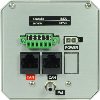
(b) 80 mm backup model until SN 21074.
