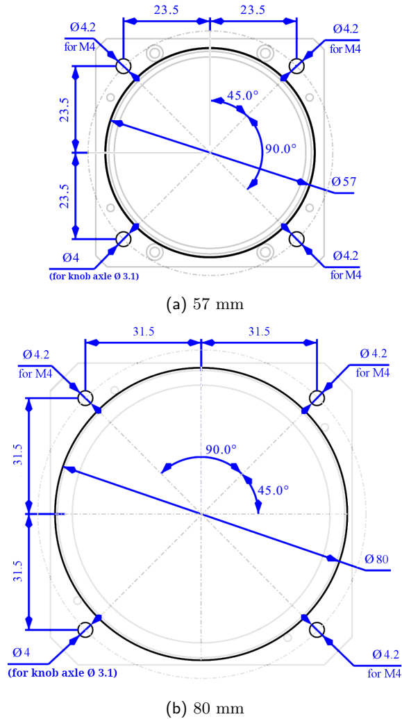
Figure 3: Instrument panel cutout and mounting hole. Note: Figure is not in scale.
