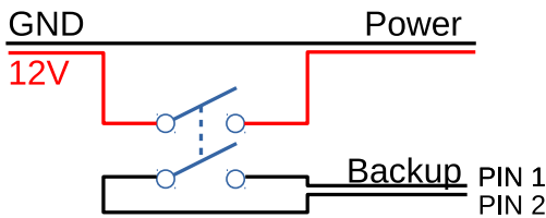
Figure 7: Connection solution with one switch controlling two circuits.
