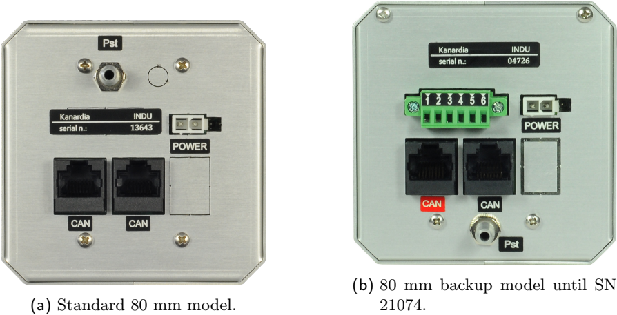
Figure 5: Back view of the 80 mm instrument with connections.
