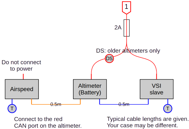
Figure 9: CAN bus power protection example. Only part connected to the orange connector is protected. The other (blue) part will shut off when system bus fails.
